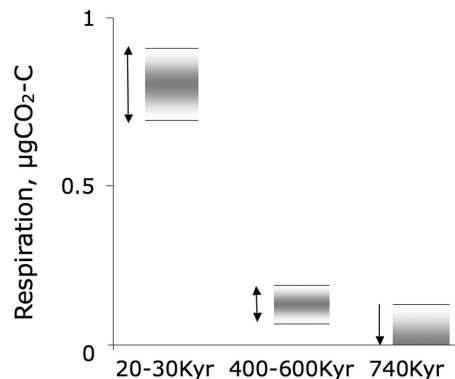
Fig. 4. Respiration in micrograms of \text{CO}_2\text{-C} per gram of dry soil per day as a function of permafrost age; the range depicted represents the minimum detectable difference by this method.
